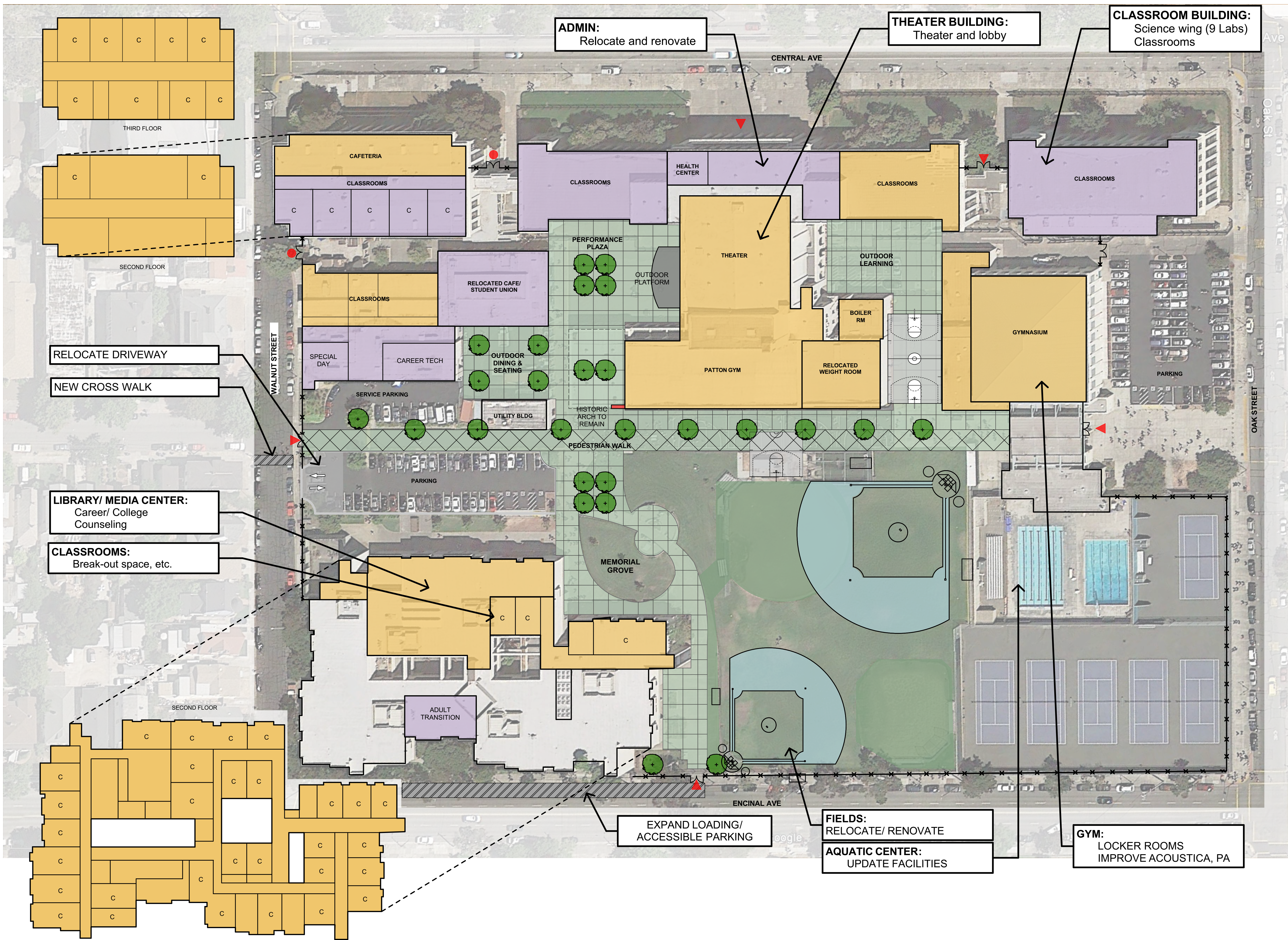
ALAMEDA HIGH SCHOOL SITE PLAN - OPTION 2
