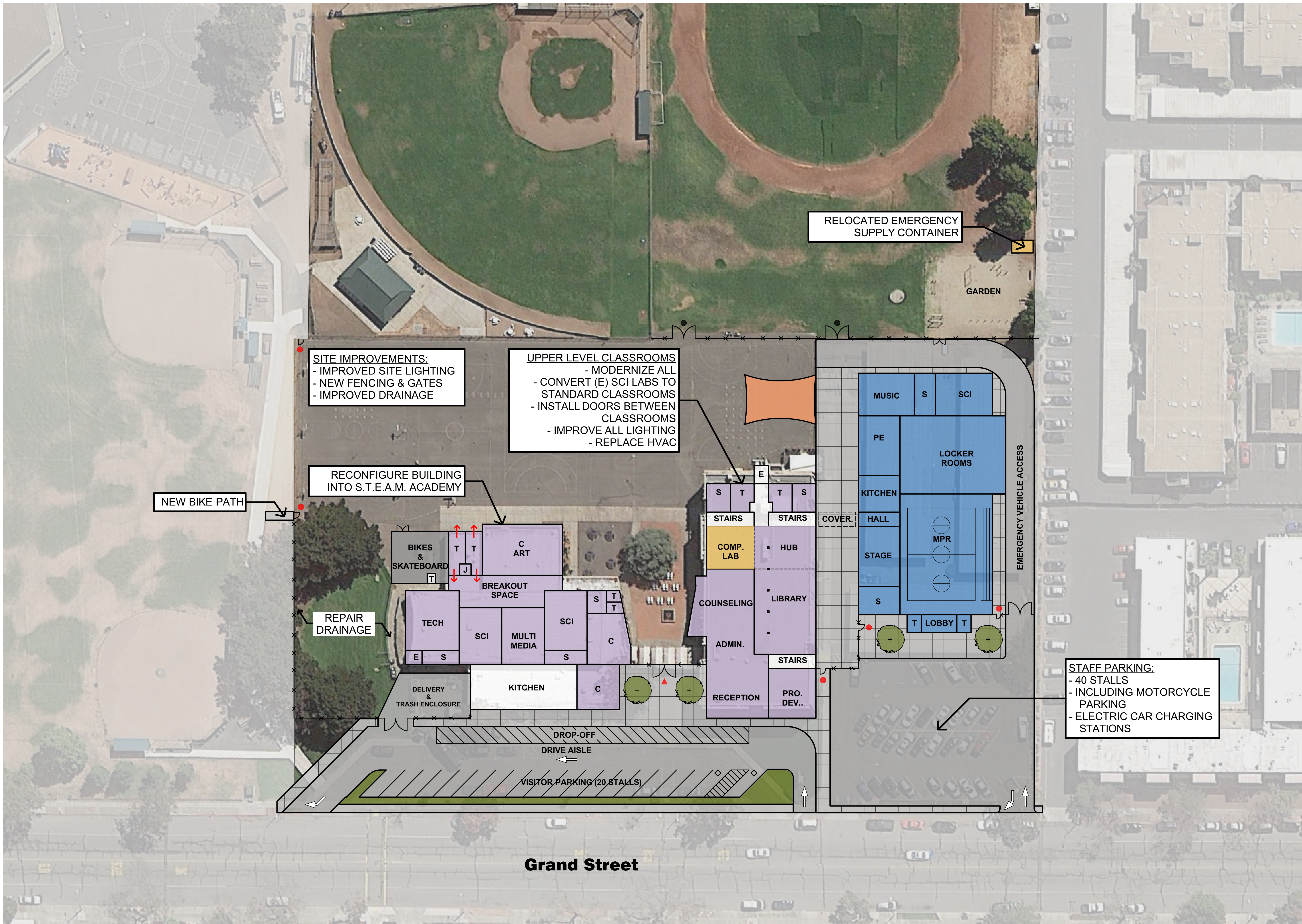
WOOD MIDDLE SCHOOL SITE PLAN
